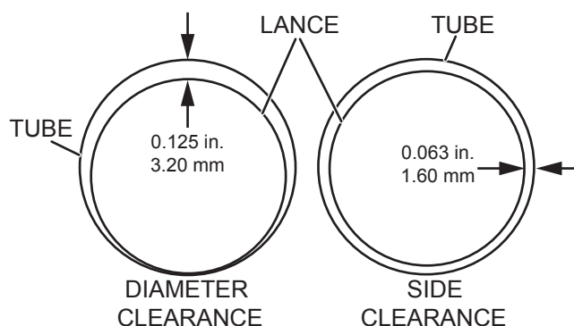
Fig. 8: Lance Clearance in Tube
