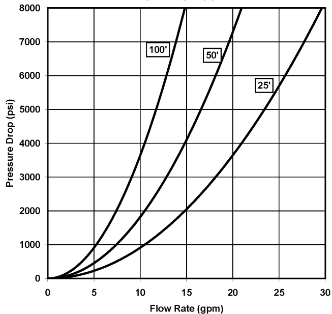
1/4" RUBBER WATERBLAST HOSE SERIES 25914
