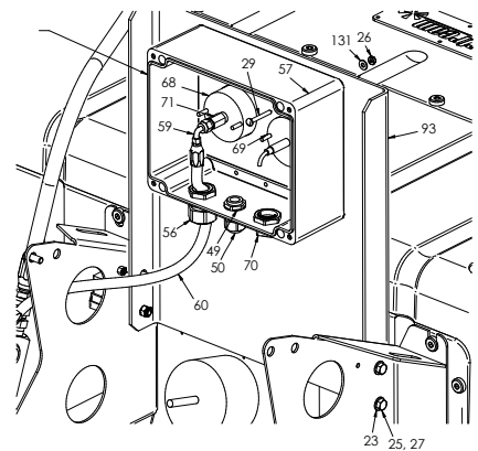
PRESSURE/TEMP GAUGE PANEL
