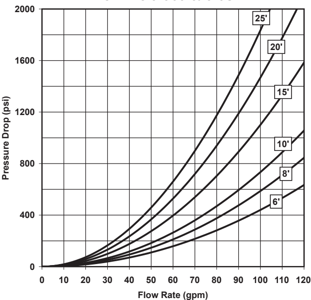
RIGID LANCES — 1/2" PIPE SERIES 51069 & 51082
