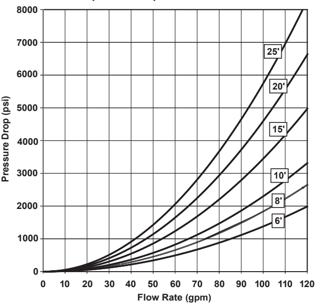
RIGID LANCES — 3/4" PIPE 15,000 PSI (1034 BAR) — SERIES 56692
