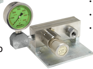
15,000 PSI Part No. 52840
