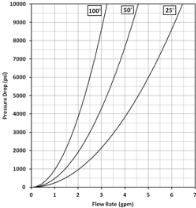
9/16" THERMOPLASTIC LANCE SERIES 28699
